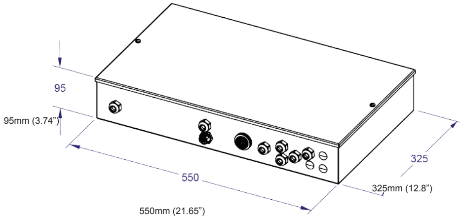
Control and Ballast Box
